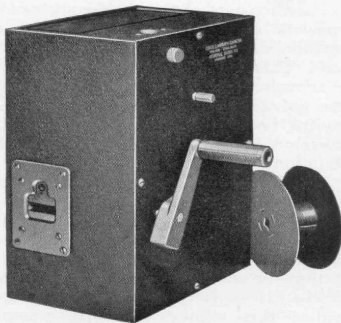
FIGURE 4. The TYPE 408 Oscillograph Camera
