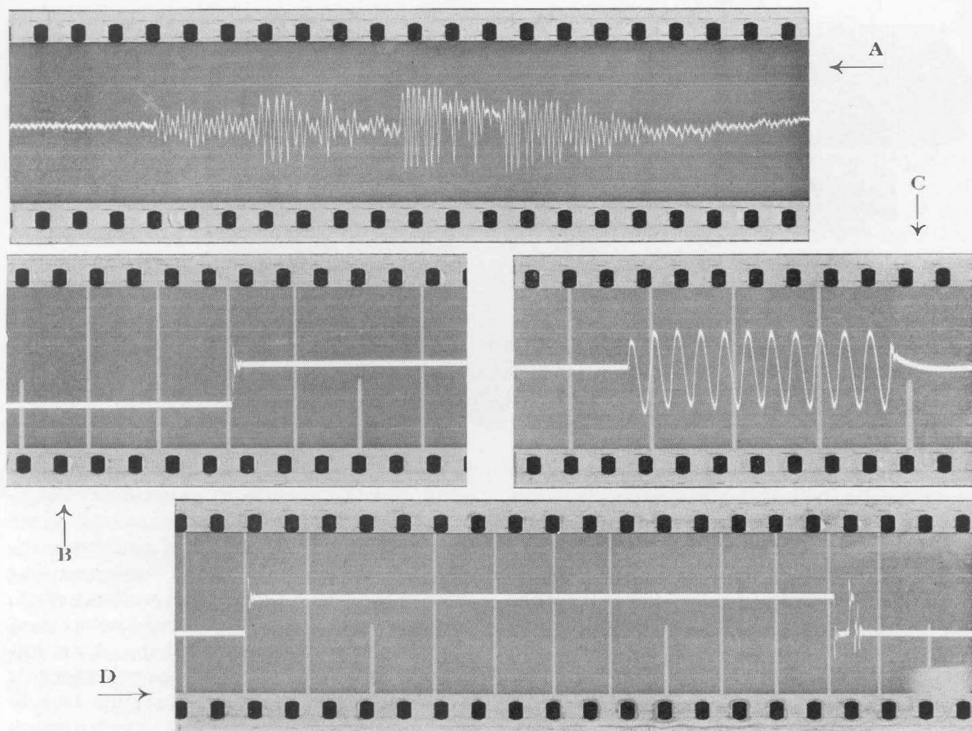
FIGURE 3. Typical records taken with the string oscillograph and camera. The vertical timing lines and the white spot (lower right corner of D ) were marked at 1/50 th-second and 1-second intervals by a synchronous shutter. A is the record of a watch tick; B and D show the operation of a relay; C shows the starting and stopping of a vacuum-tube oscillator. Time increases from left to right
