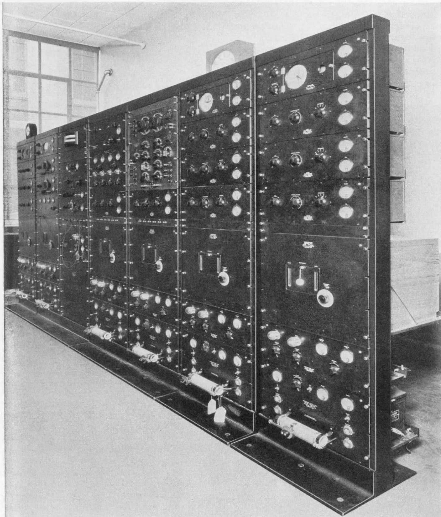
The General Radio Company's frequency-standards room. At the extreme left is a relay rack carrying the standard-frequency assembly we use for our own frequency measurements, and at the extreme right are two assemblies being tested before shipment to purchasers. The remainder is experimental equipment
